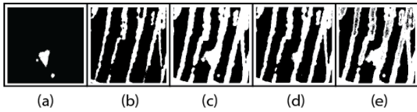
Fig. 10 Binary Images of Sample 1E from left: (a) Ground Truth Binary, and results of (b) Contrast Adjusted Thresholding, (c) MET, (d) Otsu and the (e) proposed Derivative Level Method.
