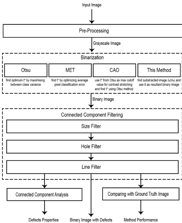
Fig. 9 Flow Diagram of the overall image processing for the defect detection.
