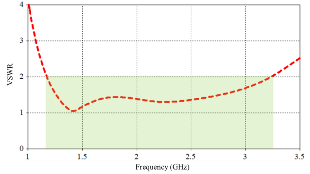
Fig. 7. VSWR (1 st antenna).
