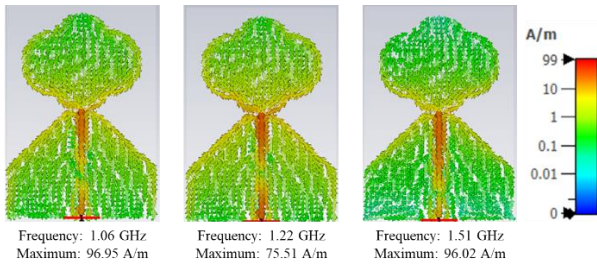
Fig. 6. Surface current distribution (2 nd antenna).
