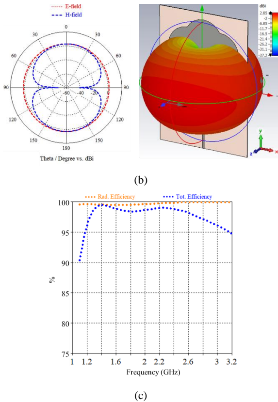
Fig. 8. 1 st Antenna radiation analysis (a) realized gain over frequency (b) 2D and 3D radiation patterns (c) efficiency.
