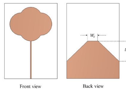
Fig. 4. Design technique (2 nd antenna).
