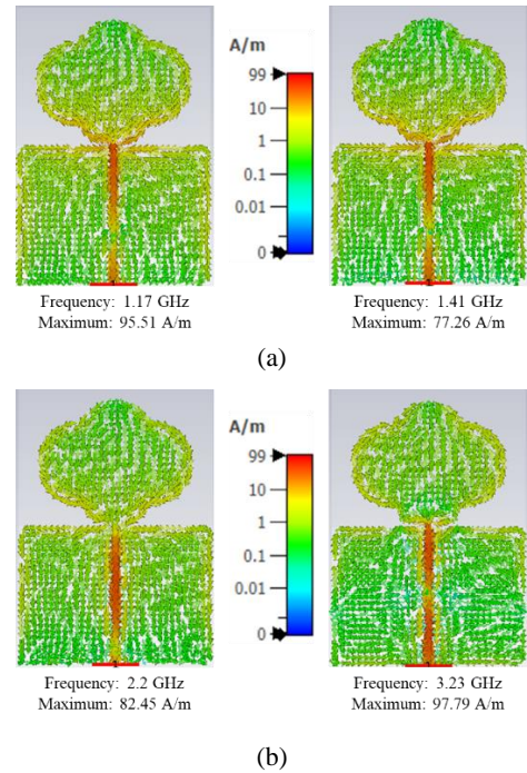
Fig. 3. Surface current distribution (1 st antenna).
