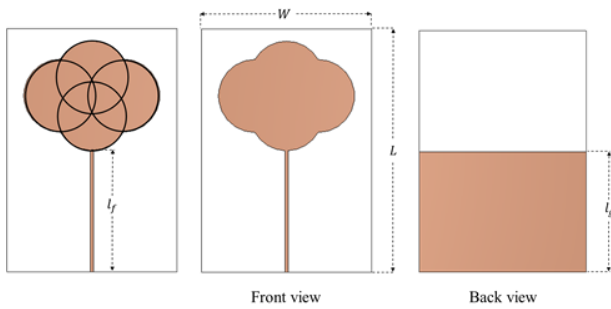
Fig. 1. Design technique (1 st antenna).
