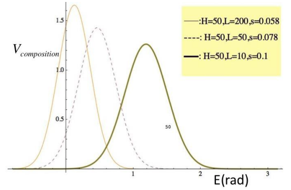
Fig.5 Examples of the proposed photographer behavior model of elevation angle
