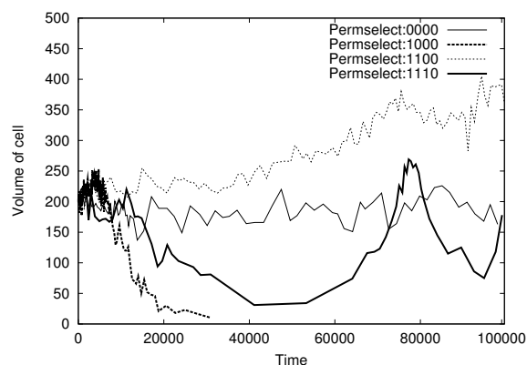
Figure 3: Examples of cell volume change as a function of time with permselectivity pattern.
