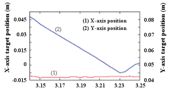
Fig. 8. Time response: target position
