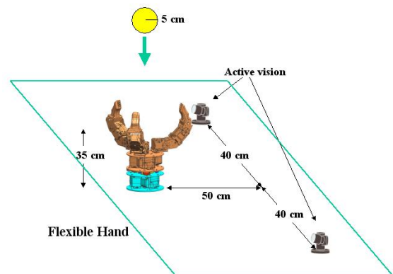
Fig. 3: Visual feedback control system
