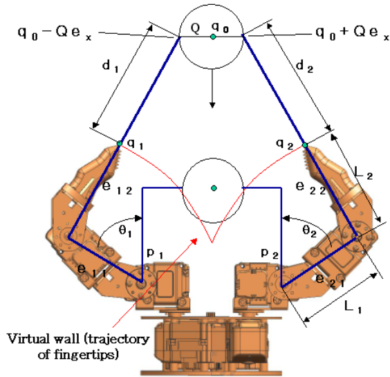
Fig. 7. Catching algorithm
