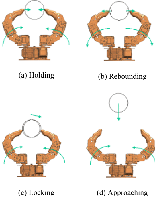
Fig. 6. Catching strategy
