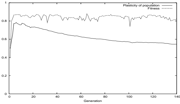
Figure 4: Fitness and plasticity of population.
