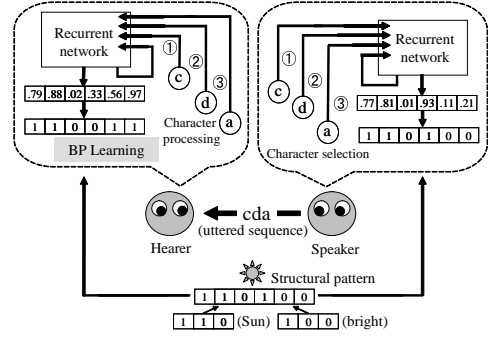
Figure 3: A communicative episode.
