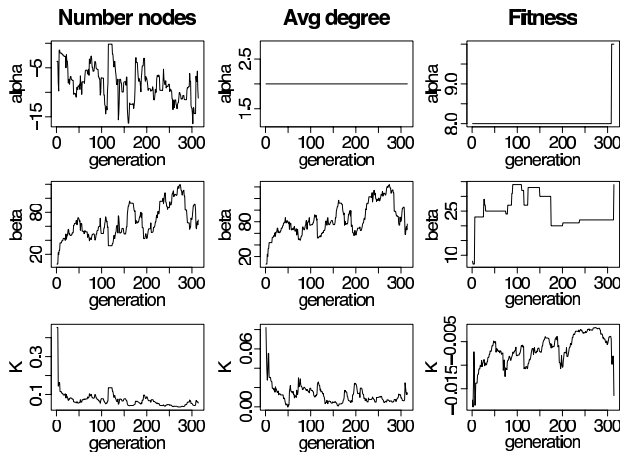
Figure 5: Evolution of the \alpha , \beta and K parameters for the winning lineage on all traits.
