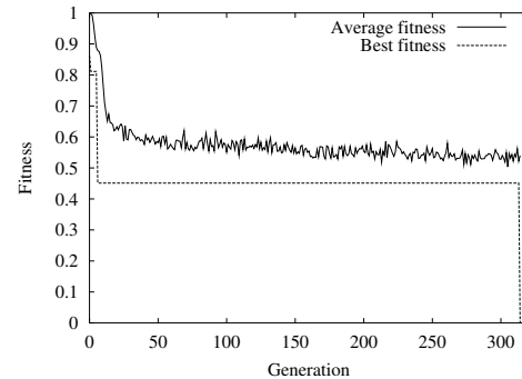
Figure 2: Fitness graph for a typical run.
