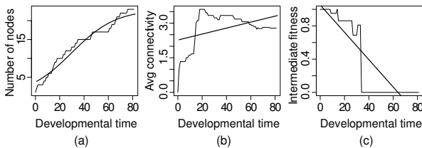
Figure 4: Growth curves for the analyzed traits on the best individual. Both growth data and fitted curves are shown. For the number of nodes, a sigmoidal curve was fitted, while simple linear regression was used for the other traits.
