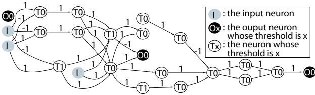
Figure 3: The best neural network for the run. Please note that the cellular encoding model may produce more inputs and outputs than necessary, as it can be seen in this case, although only one output is actually used. The output node in the center is the used one.
