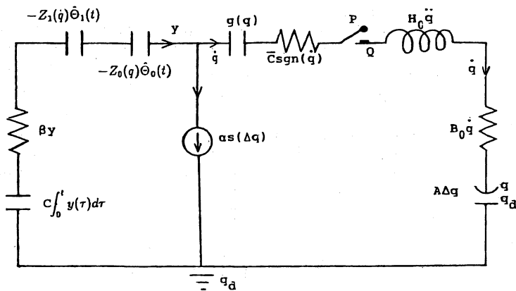
Fig. 6 A circuit expressing dynamics of single degree of freedom under static and Coulomb's frictions.
