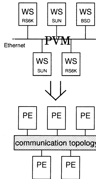
Figure 2: Parallel Virtual Machine
