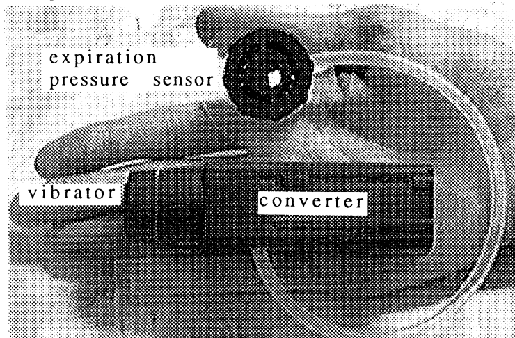
Fig.6. Electric artificial larynx
