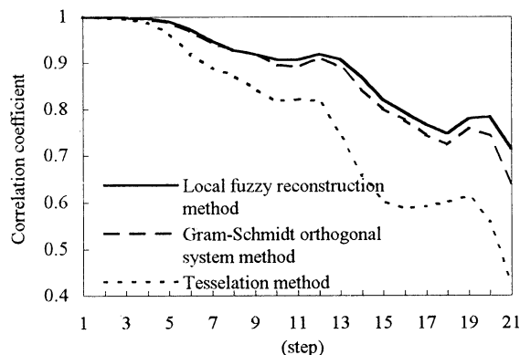
Fig. 6 Predictability in Lorenz system
