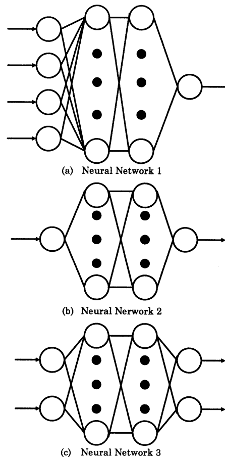
Fig.2 Neural Networks in ABrain
