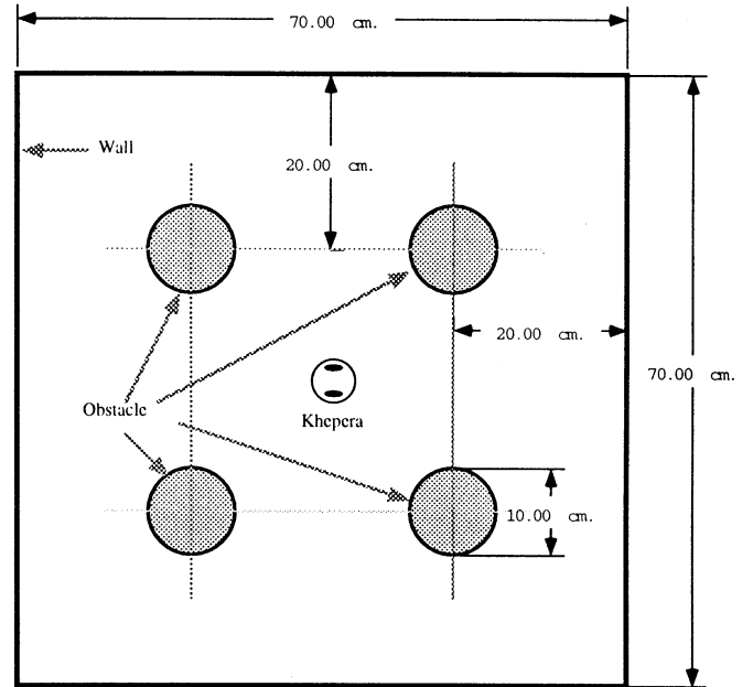
Figure 3: Simulation field
