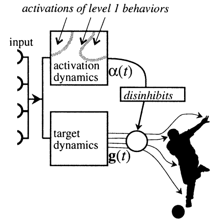
Figure 1: (a) Global structure of a DD behavior control system. At any time, every behavior has an activation. Activations of higher-level behaviors (depicted in shaded boxes) act as control parameters for the activation dynamics of lower levels. The dynamical system which maintains a behavior’s activation can undergo bifurcations; this is indicated by depicting these systems as stylized “phase diagrams” (boxes with irregular partitions). A mode of the entire system is thus determined by the activations of all higher-level behaviors. (b) The target and activation subsystems of an elementary behavior.
