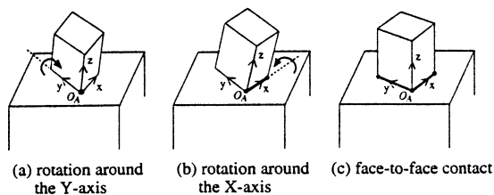
Fig.2 Rotate-to-level skill
