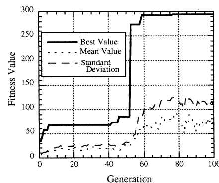
Figure 9: Result of evolution in only PE 3
