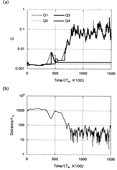
Figure 4 Learning for approaching the attractant. T_m is the period of motor rotation. (a) Q -functions. The number after Q in the legend correspond to the rule number in Table 1, (b) Distance between the robot and the attractive material.
