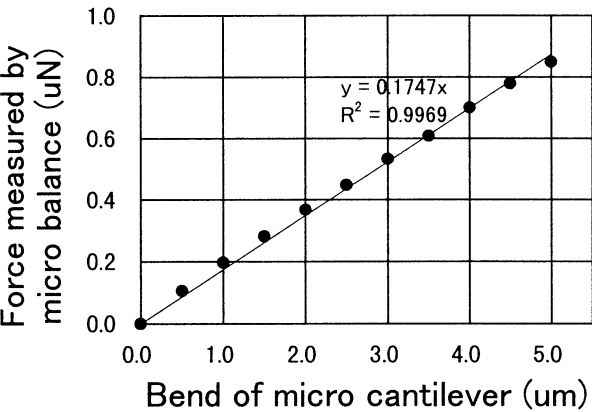
Fig. 6 Spring constant of micro cantilever
