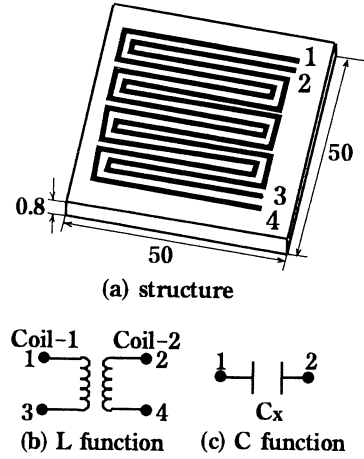
Fig. 5: Structure of the comb shaped mono-structural touch sensor
