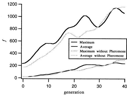
Fig.3 The progress of the fitness according to the evolution.
