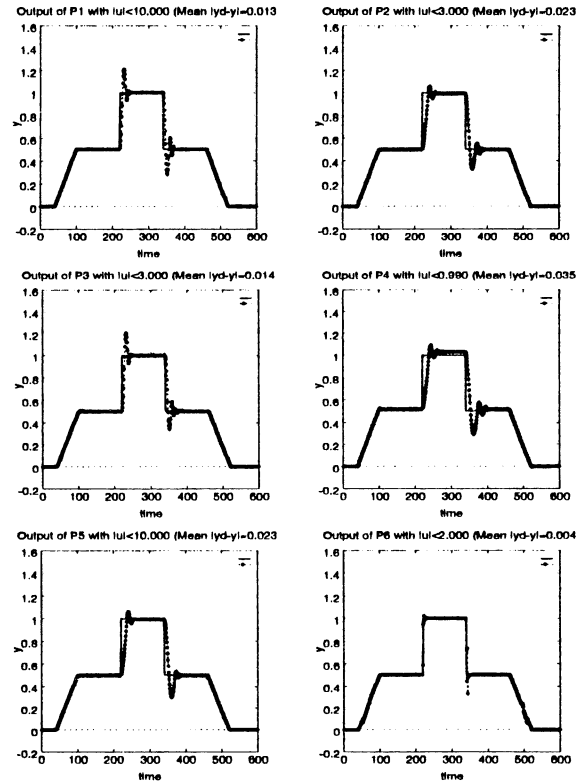
Figure 3: The output of the plants p_1, p_2, \dots, p_6 controlled via the predictive controller with CAN2.
