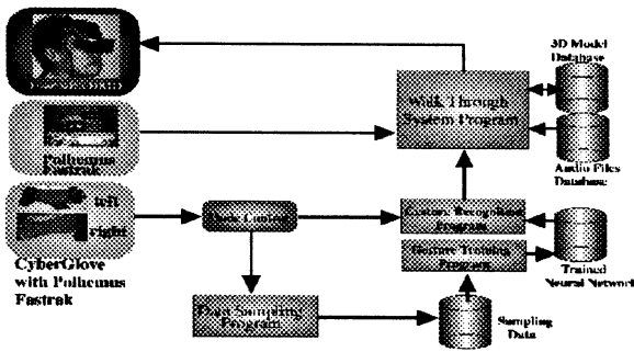
Figure 3: System Architecture
