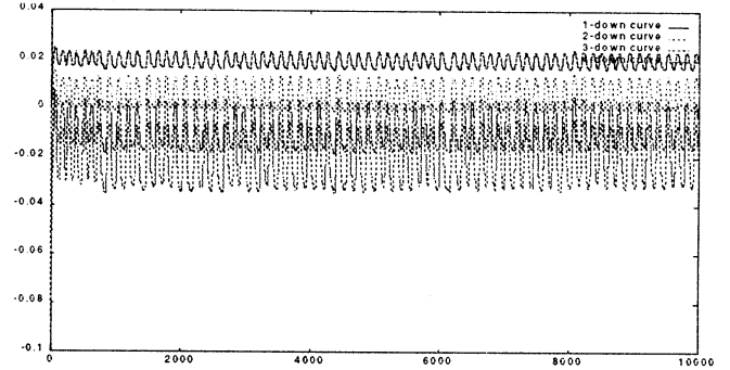
Figure 3-(2b) The n-down curves ( n=1,2,3,4 ) for \ell=1 , a=0.030 , b=0.034 .
