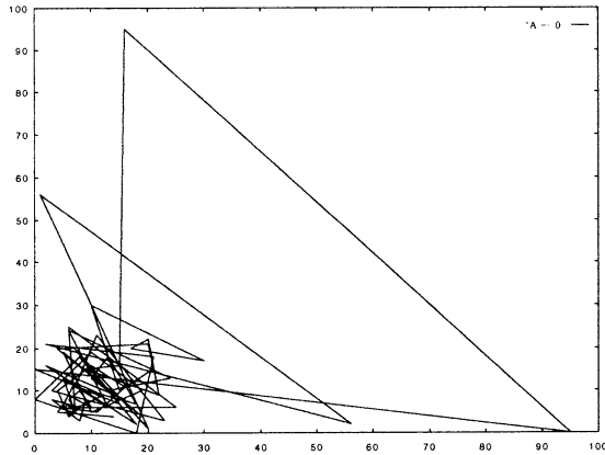
Figure 1(a) (x_i^k, x_{i+1}^k) plot of intervals of '0' for A..
