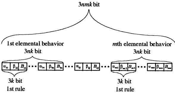
Figure 3: Individual structure
