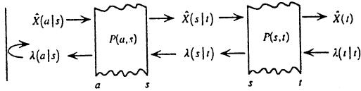
Figure 3. Internal state.
