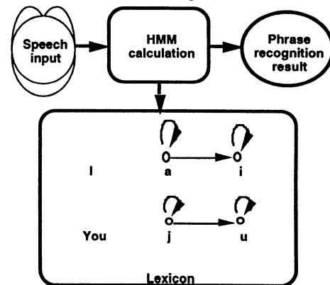
Fig. 4 Phrase recognition
