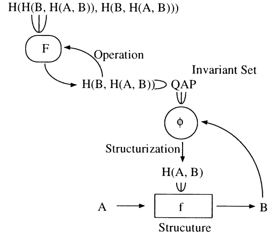
Figure 2: Quasi-Autopoietic Systems
