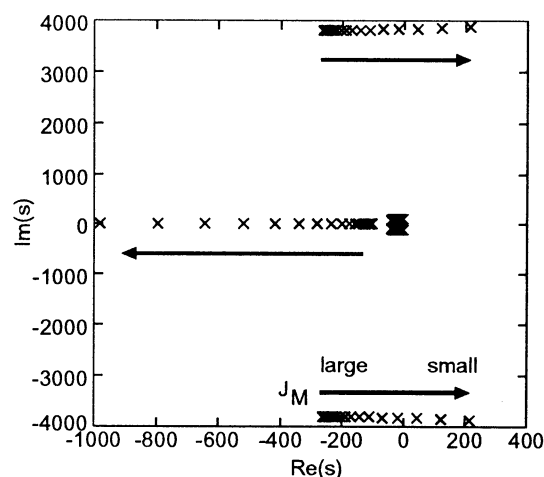
Figure 4: Relationship between motor inertia J_M and poles of the 6th order model for the industrial robot manipulator
