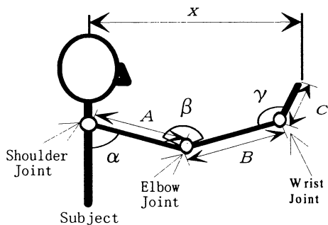
Fig. 3 The concept of the arm angles sensor
