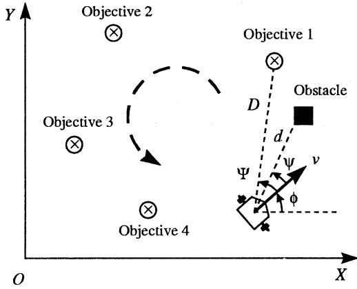
Figure 9: Behavior model for a mobile robot with two independent driving wheels
