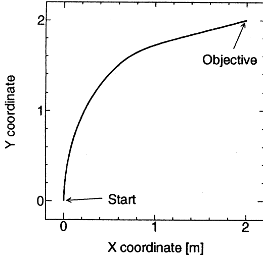
Figure 4: Resulting mobile robot path
