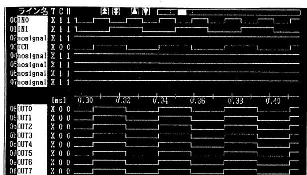
Figure 8: Signals in the experimental MNN on FPGA erators and 50% (398 of 800) CLB flip-flops.
