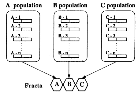
Figure 3: Coding of individuals and the composition of populations
