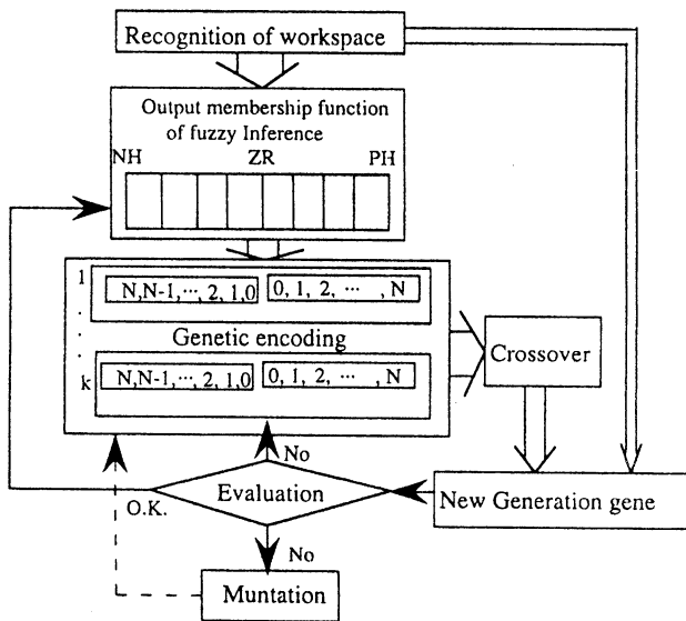
Fig.2 Combined operation of fuzzy-genetic algorithm.
