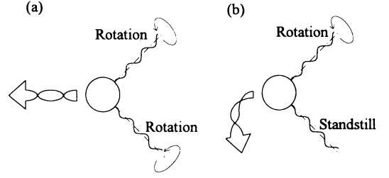
Figure 2 Moving modes of the robot. (a) Mode 1, screws are rotating in the same direction and the robot moves almost straight, (b) Mode 2, one screw stops while the other keeps rotating, and the robot turns.
