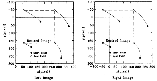
Fig. 5 Trajectories of the feature points on the images.
