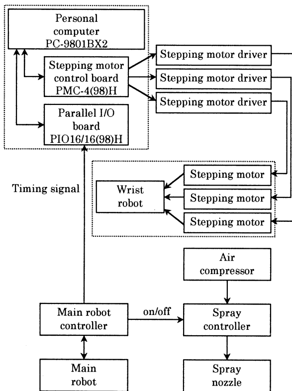
[Fig.4-1] System for spray test
