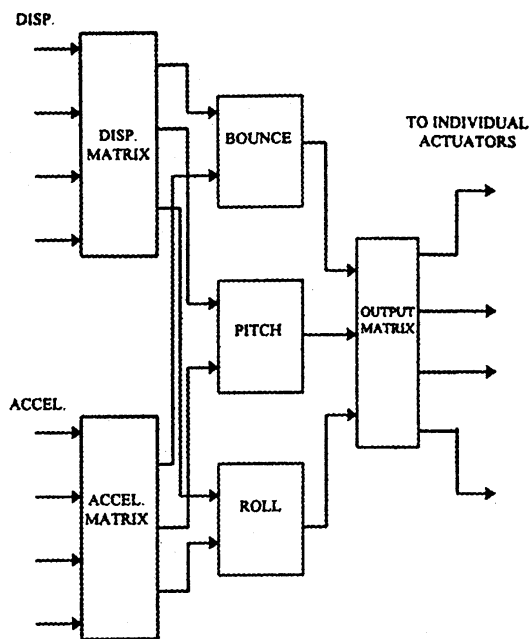
Figure 2 Modal Controller
