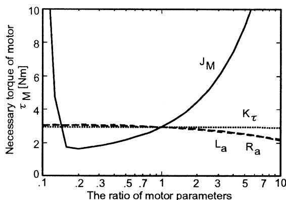
Figure 3: Relationship between the ratio of motor parameters and the necessary torque of the motor
