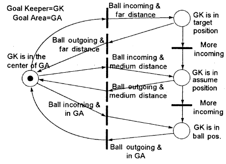
Figure 13: Petri-net model of goal keeper controller.
