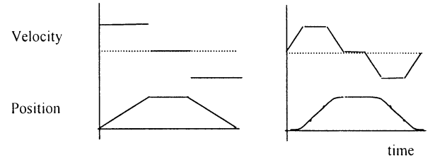
Figure 2. Position and velocity profiles for kinematic and dynamic systems
