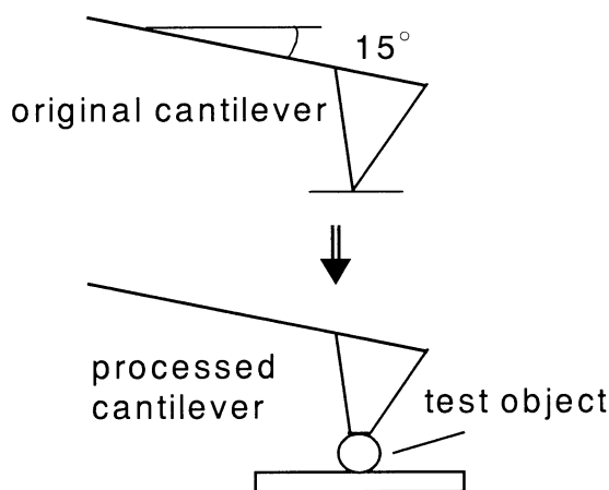
Fig. 2 AFM tip processed to make flat contact by FIB
