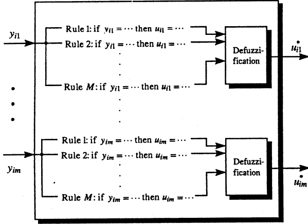
Figure 3: Internal fuzzy rules for a behavior group i
