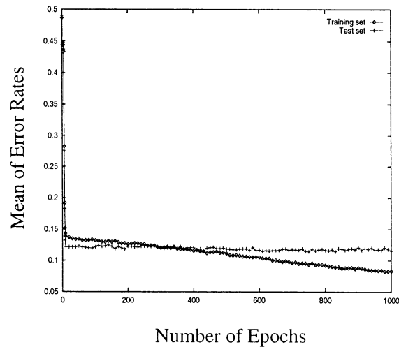
Figure 1: The average result over 25 runs of our ensemble learning algorithm for the Australian credit card assessment problem. The horizontal axis indicates the number of training epochs. The vertical axis indicates the error rate.
