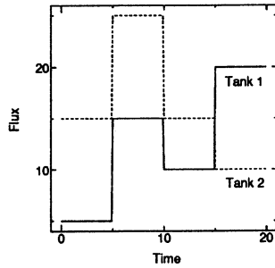
Fig.4 Outflows of the 1st & 2nd holonic subsystem
