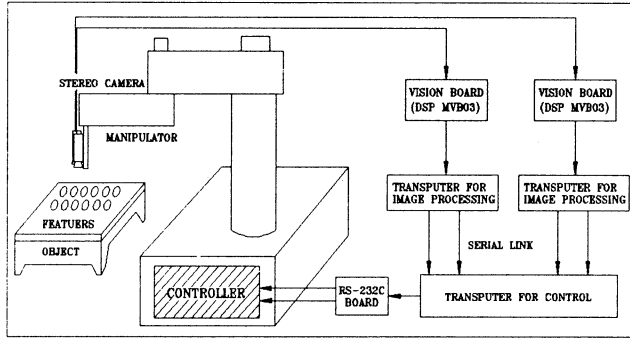
Fig. 1 Schematic diagram of visual servoing system
