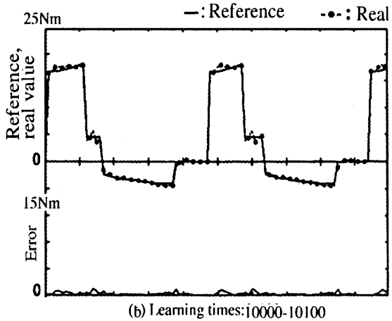
Fig.6. Torque control results where (a) shows the initial stage and (b) shows the final stage.
