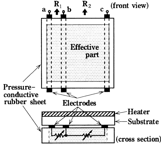
Fig. 1: Structure of a mono-material pressure-conductive rubber sensor with two output signals
