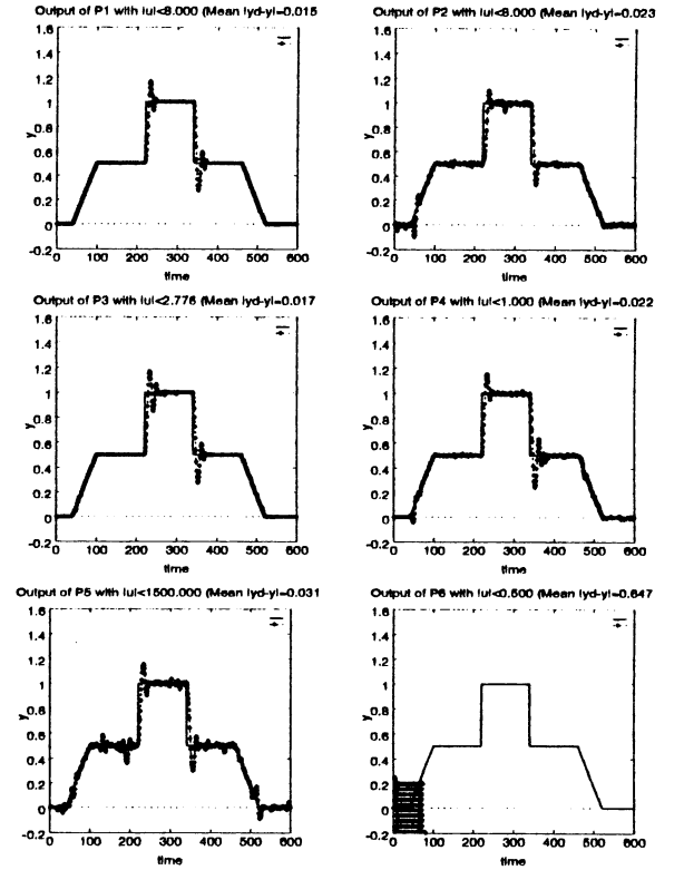
Figure 1: The output of the plants p_1, p_2, \dots, p_6 controlled via the inverse controller with CAN1.
