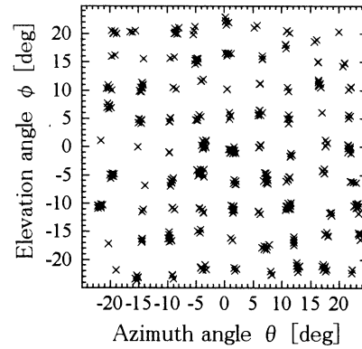
Fig.6 Accuracy of pointing by using four LED marks
