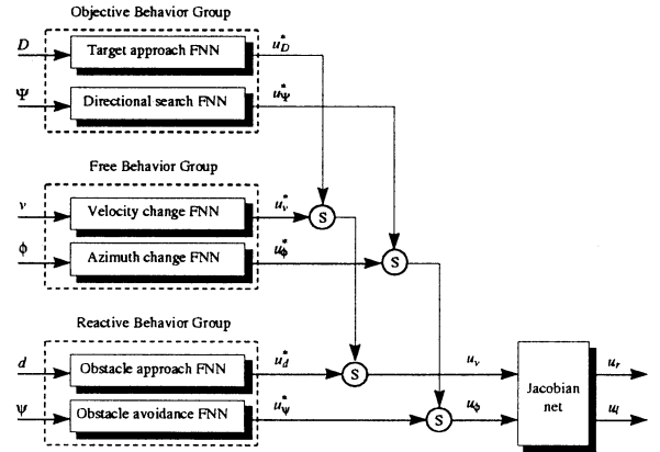
Figure 10: Fuzzy behavior-based control system for a mobile robot
