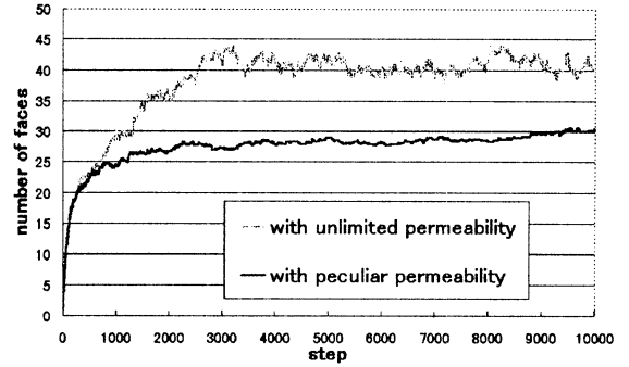
Fig.2 The average of number of faces in the system (The value in this figure is average of five trials)
