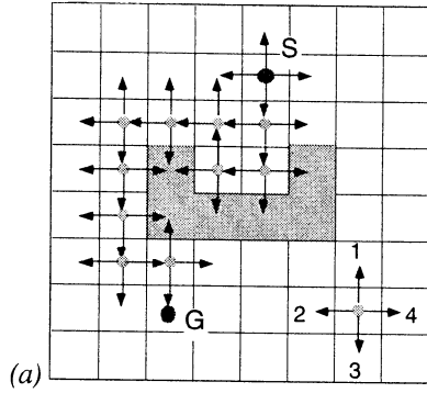
Figure 1: (a) A*-search in the implicit C-space from the start configuration S to the goal configuration G , (b) collision detection by distance computation in the workspace
