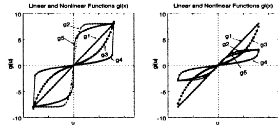
Figure 4: The ranges of the function values g_i(u) for the inverse (left) and the predictive (right) controller where x is normalized.
