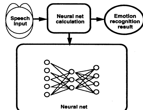
Fig. 5 Emotion recognition
