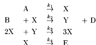
Figure 2: Abstract chemical model of Brusselator.
