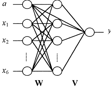
Fig.1 BP model
