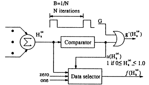
Figure 4: Neuron unit
