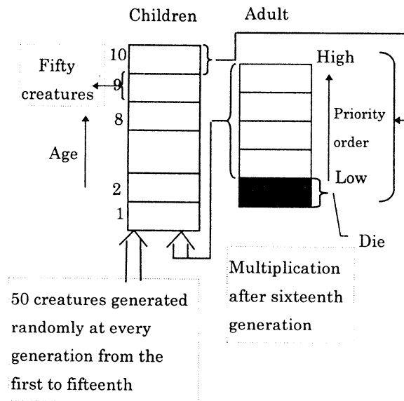
Fig.4 Creature's multiplication
