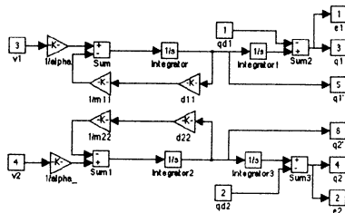
Figure 2: The internal model via SIMULINK.
