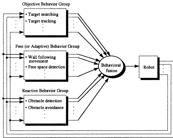
Figure 1: A behavior-based control system using multiple behavior groups for a mobile robot
