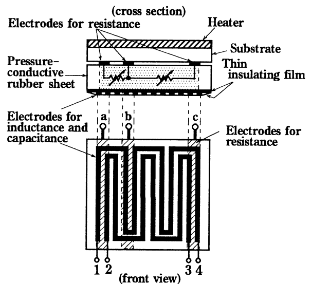
Fig. 7: Compound multi-functional robot-hand tactile sensor
