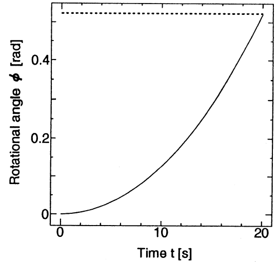
Figure 5: Resulting rotational angle of robot
