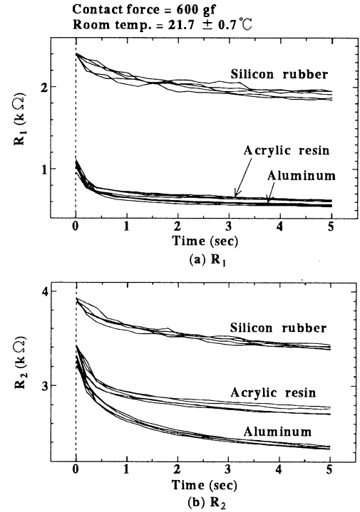
Fig. 3: Time responses of R_1 and R_2 of rubber sensor after contact with materials
