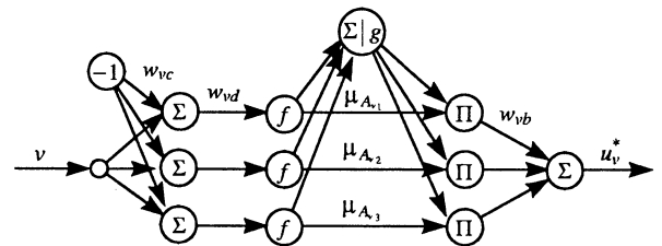
Figure 11: A FNN for an elemental behavior
