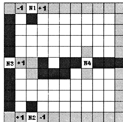
Fig 3 The structure which can be used to solve the XOR problem. The gray grids represent the axon cells and the dark cells the dendrite cells. -1 means that the axon trail the signal by -1 while +1 means the axon pass down the signal without change.
