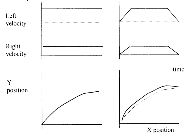
Figure 3. Left and right wheel velocity profile and curved path for kinematic and dynamic models
