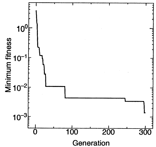
Figure 6: History of minimum value of fitness
