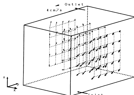
Fig.10 Velocity distribution in a chamber
