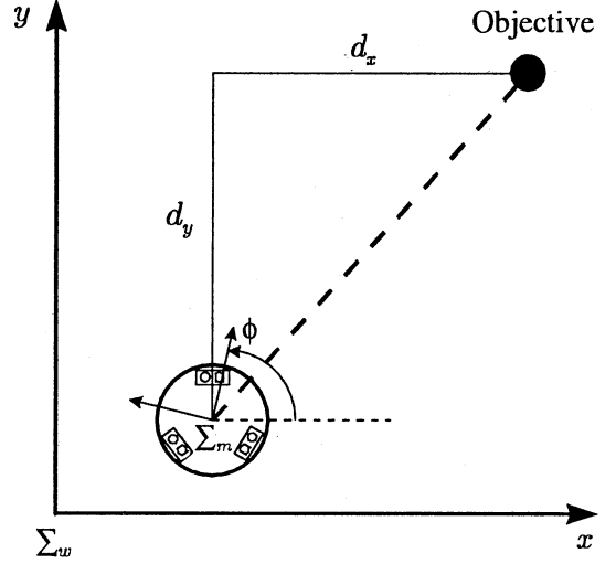
Figure 1: Behavior model for an omnidirectional mobile robot
