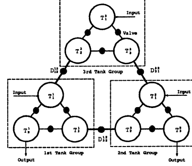
Fig.2 Tank network system
