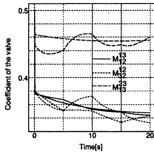
Fig.5 Result of conventional holonic control system
