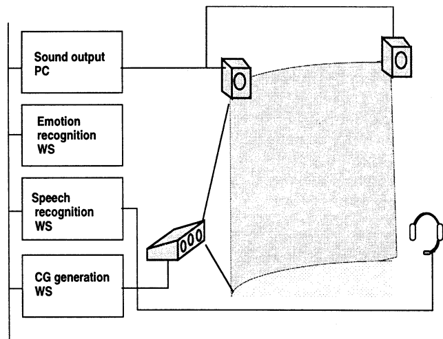
Fig. 7 Interactive Poem hardware configuration
