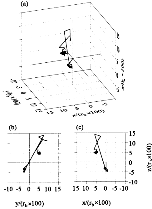
Figure 5 Trajectory of the robot approaching the attractant at (500, 500, 500). The robot starts from the origin. (a) Bird's-eye view, (b) Cross-sectional view; y-z plane, (c) Cross-sectional view; x-z plane.
