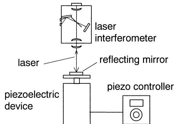
Fig. 3 A laser interferometer to measure deformation of piezoelectric device
