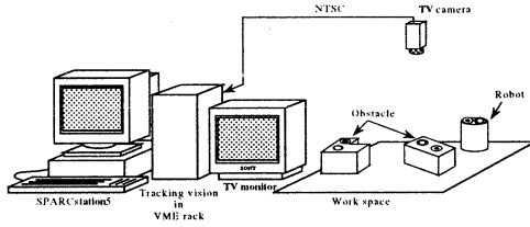
Fig. 5: Experimental equipment.
