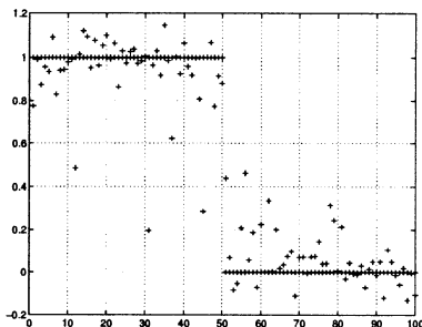
Figure 8: real and expected outputs of BP2 [with open data]
