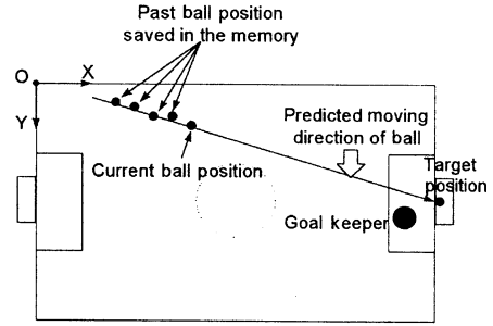
Figure 12: Subroutine 'predictor()'.
