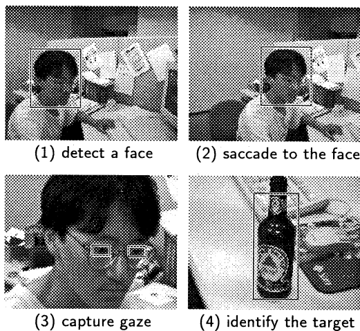
Figure 6. Gaze-monitoring process
