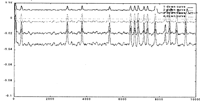
Figure 3-(1b) The n-down curves ( n=1,2,3,4 ) for \ell=1 , a=0.030 , b=0.027 .
