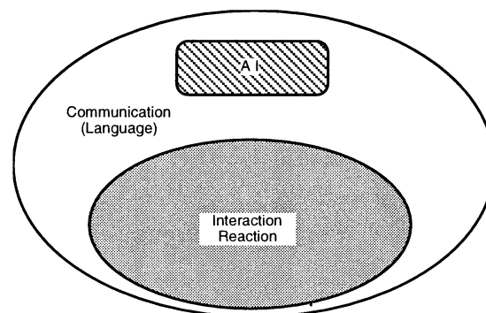
Fig. 1 Communication Model
