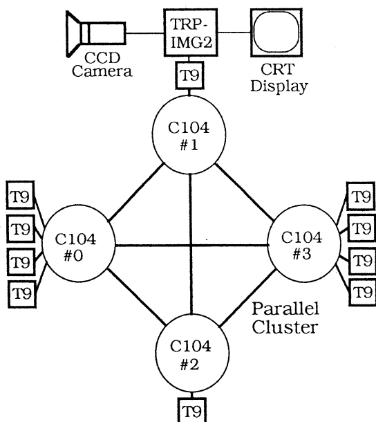
Fig.5 Configuration of Experimental System
