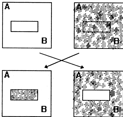
Fig. 2. Crossover operations
