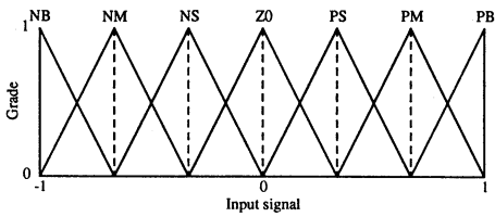
Fig. 2: Membership functions.
