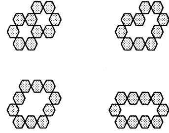
Figure 2: Deadlock states
