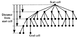
Fig. 4: Tree.
