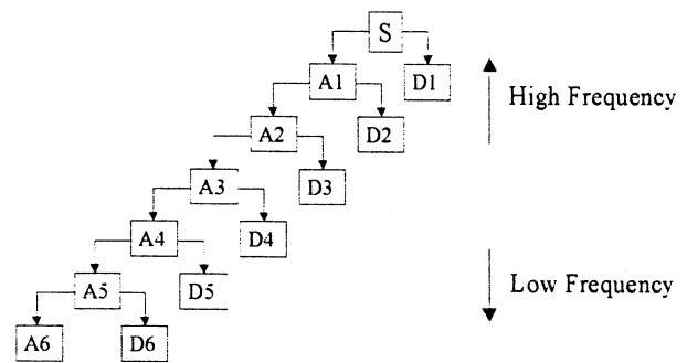
Figure 3. Multi-Level Decomposition
