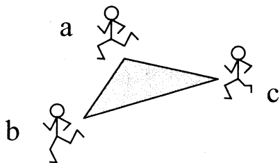
Figure 6 The relationship between three players represented by a triangle (2-simplex).
