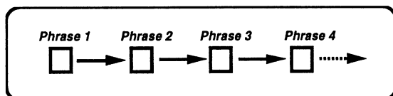
Fig. 2-A Conventional poem
