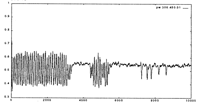
Figure 3-(3a) The average price for \ell=1 , a=0.030 , b=0.045 .
