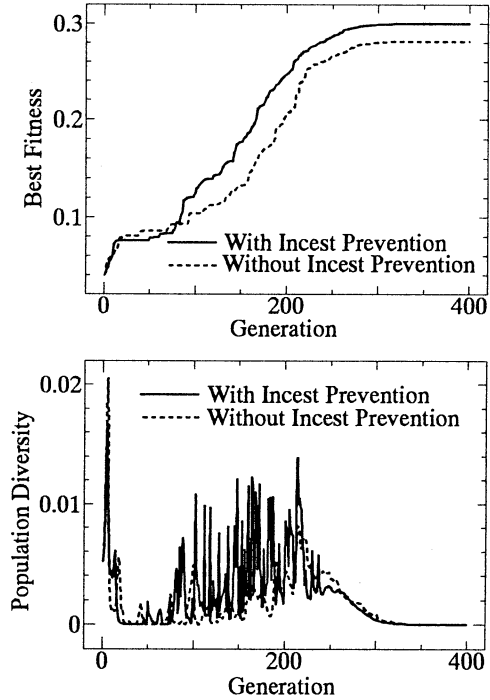
Figure 3: Evolutionary results
