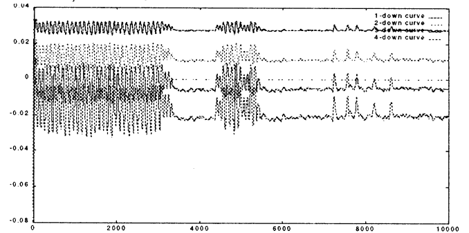
Figure 3-(3b) The n-down curves ( n=1,2,3,4 ) for \ell=1 , a=0.030 , b=0.045 .
