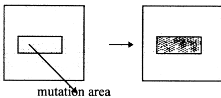
Fig. 3. Mutation operation
