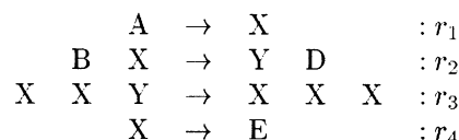
Figure 3: Rewriting rules for Brusselator.
