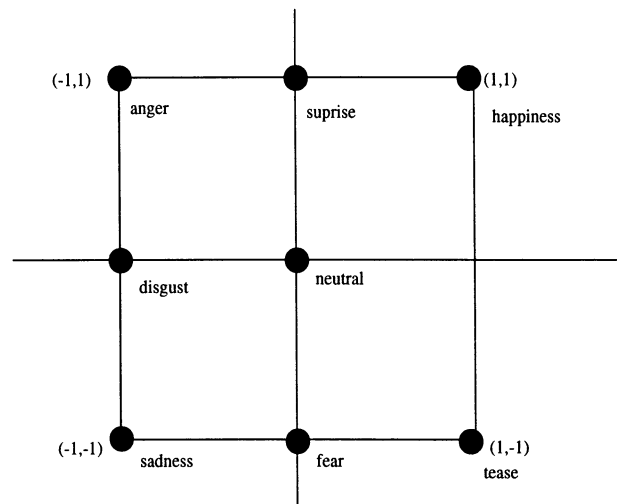
Fig. 11 Emotional plane
