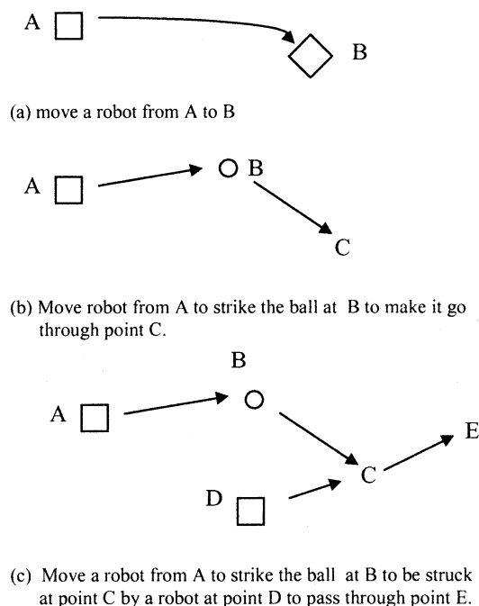
Figure 2. Benchmark Problems
