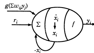
Fig. 1 Dynamic Neuron
