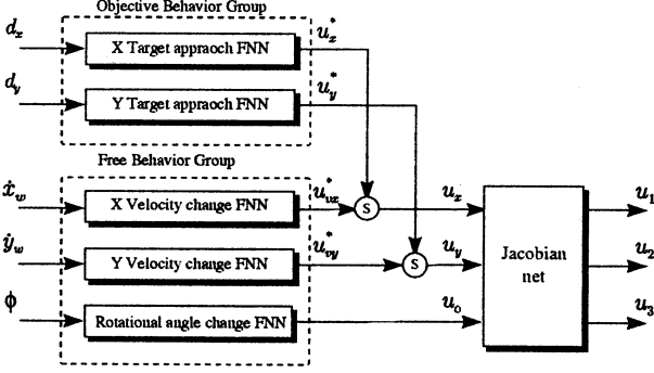
Figure 2: Fuzzy behavior-based control system
