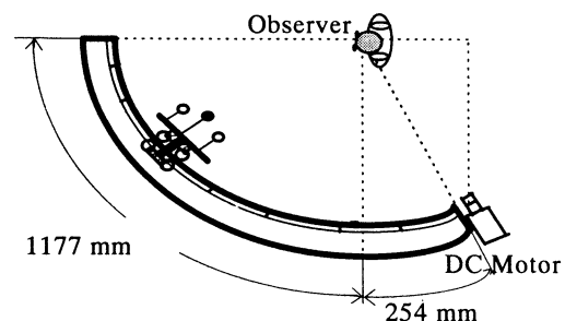
Fig. 5 mechanism of the movable targets
