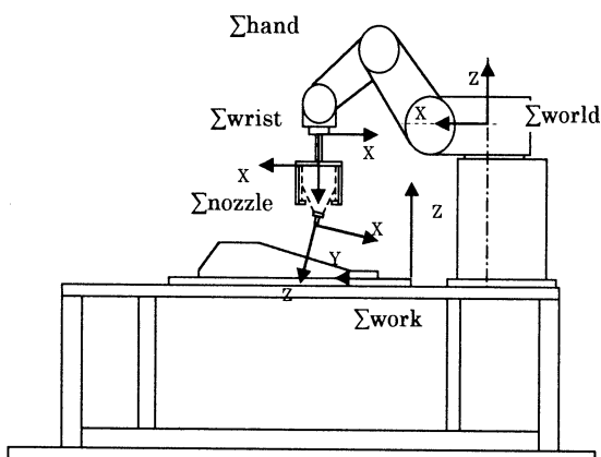
[Fig.4-2] Relation of coordinates in test system
