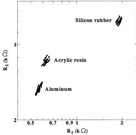
Fig. 4: Two-dimensional explanation of R_1 and R_2 of pressure-conductive rubber sensor
