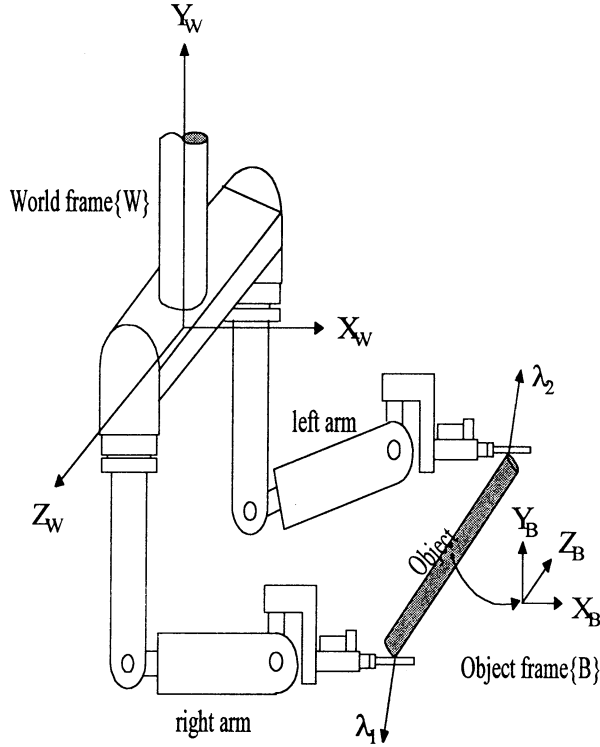
Figure 1 Dual Arm Manipulator, RM-10A
