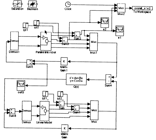
Figure 3: Feedback configuration of the parallel link robot manipulator with PID+Q controller.
