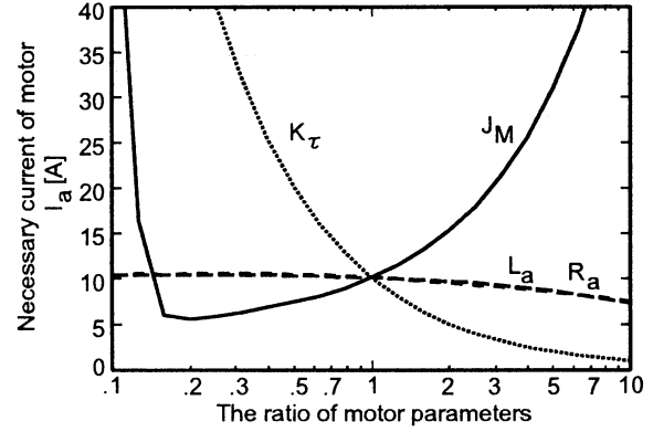
Figure 2: Relationship between the ratio of motor parameters and the necessary current of the motor
