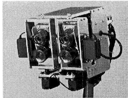
Figure 5. The attention-sharing robot
