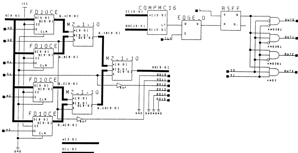
Figure 7: Circuits inside of the control unit
