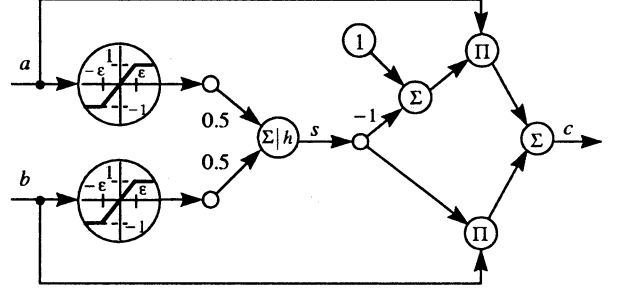
Figure 7: Saturation function-type suppression unit realized as a NN
