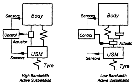
Figure 1 Active Suspensions
