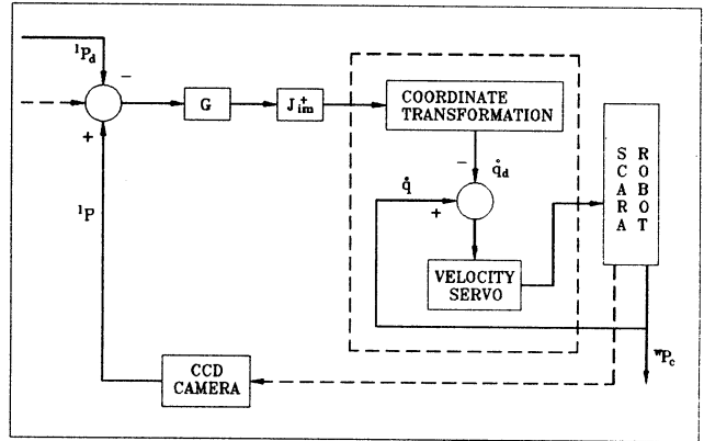
Fig. 3 Block diagram of visual feedback system.
