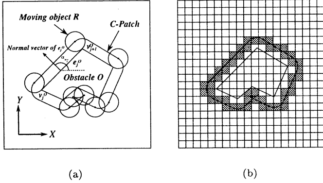
Fig. 3: Representation of an obstacle in C-space in case a robot is circle.
