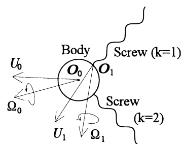
Figure 1 Micro-robot imitating bacteria. The two screws rotate and propel the body. The radius of the body is r_b .
