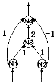
Fig 2 The structure and weight of EQUnn model which can be used to solve the XOR problem. N1, N2 represent the input neurons, N3 the hidden layer neuron and N4 the output neuron.
