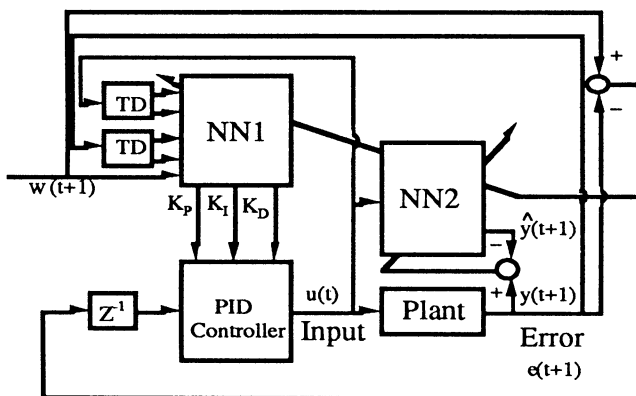
Fig. 3. Neuro-PID controller configuration.
