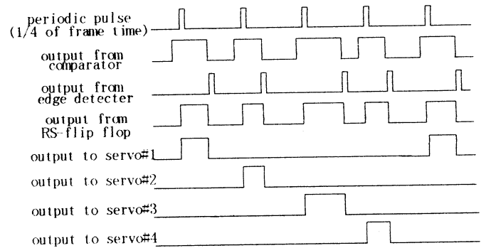
Figure 8: Timing chart of the signals
