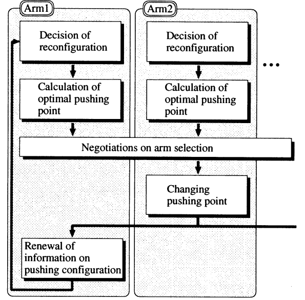
Figure 2: Outline of changing pushing points.
