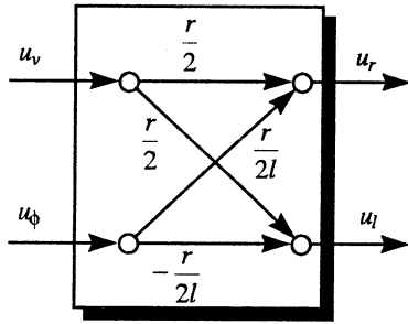
Figure 12: Jacobian net: known case
