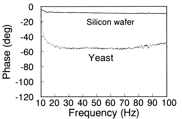
Fig. 7 Phase shift of deformation of dry yeast and silicon wafer detected by the dynamic viscoelasticity measurement system
