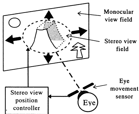
Fig. 3 The concept of wide view HMD
