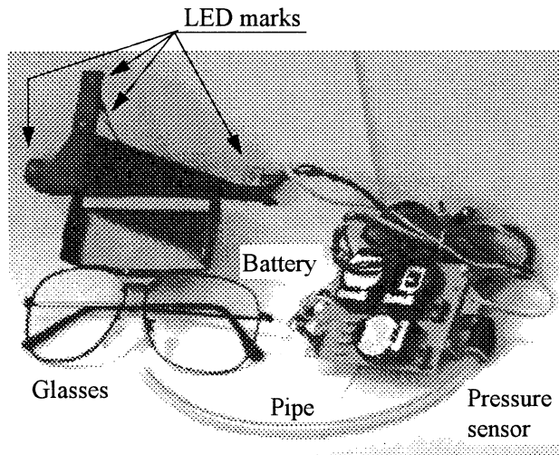
Fig. 2 Glasses with three LED marks
