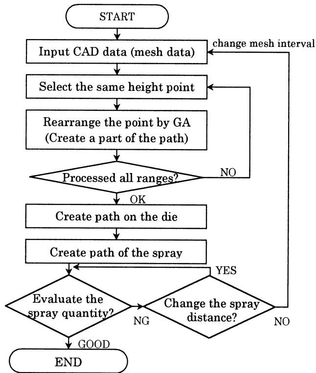
[Fig. 3-1] Path calculation flow chart
