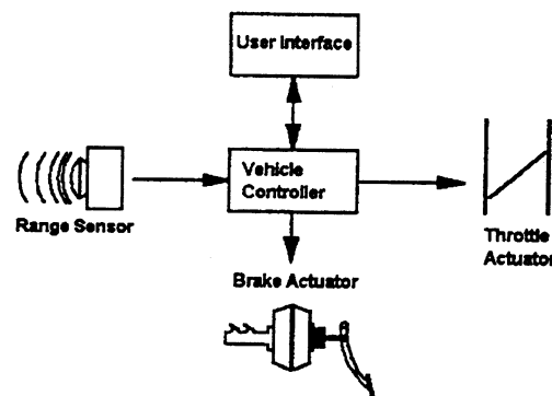
Figure 4 ACC system components
