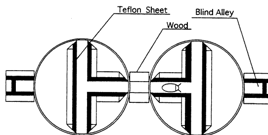
Fig.5 Apparatus with teflon walls and blind alleys.
