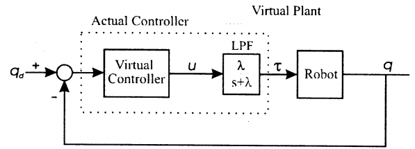
Fig. 1. Block Diagram of the Virtual System
