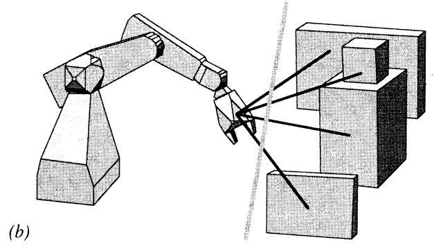
Figure 1: (a) A*-search in the implicit C-space from the start configuration S to the goal configuration G , (b) collision detection by distance computation in the workspace
