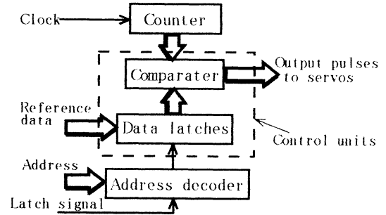
Figure 5: Block diagram of the circuits in FPGA
