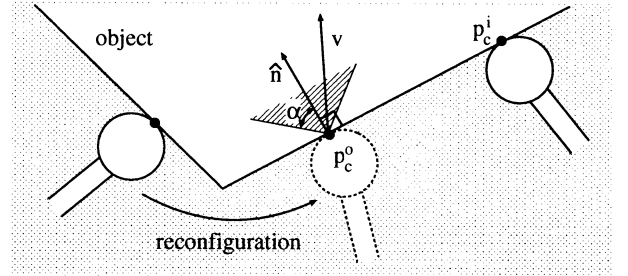
Figure 3: Changing pushing point.
