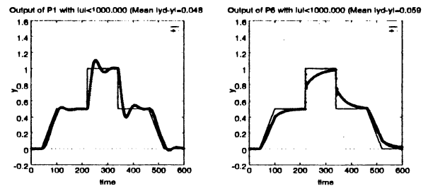
Figure 5: The output of the plants controlled via the PID controller with K_P=4.5 , K_I=0.1 , K_D=10 for p_1 , and K_P=2 , K_I=0.1 , K_D=0.1 for p_6 .
