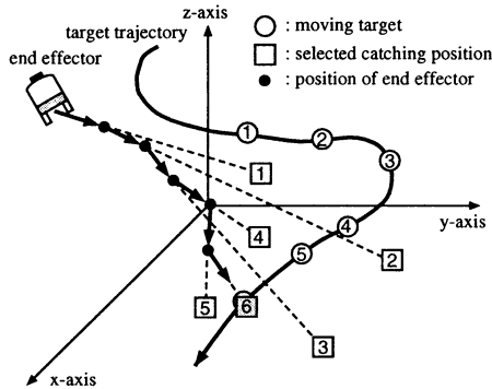
Fig. 4: Catching motion of the robot manipulator.
