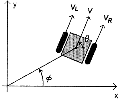
Figure 1: Modeling of kinematics.
