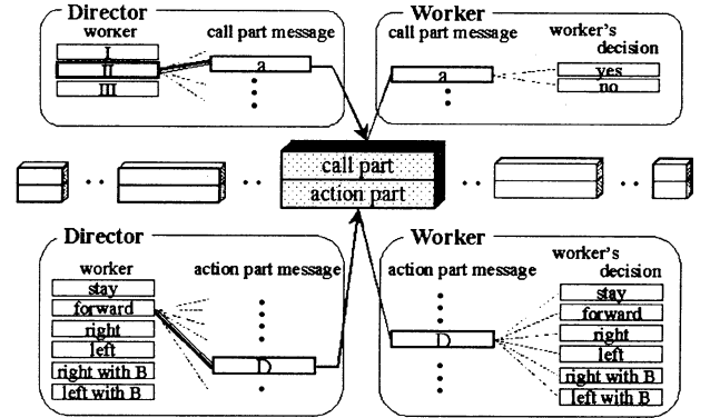
Figure 2: The structure of message
