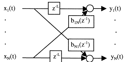
Fig. 1 Signal Separation Network
