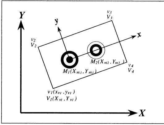
Fig. 2: Parameters for the geometric object model.
