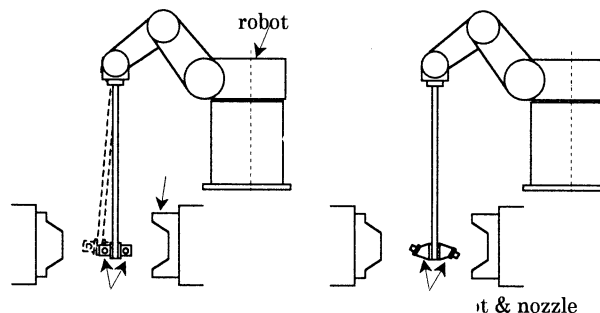
[Fig.2-1] Spray robot layout
