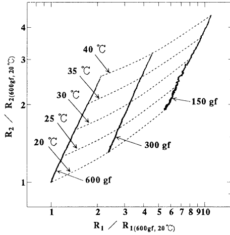
Fig. 2: Temperature characteristics in three kinds of contact forces
