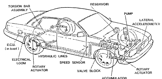
Figure 3 ARC installation
