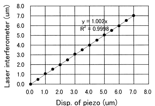
Fig. 4 The linearity of piezo electric device deformation
