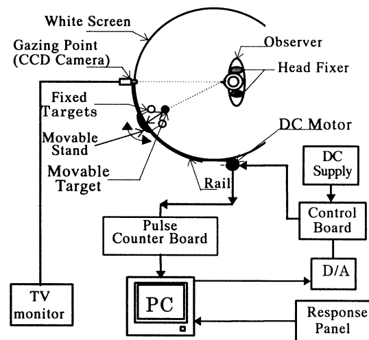
Fig. 4 Schematic diagram of the experimental system to measure the kinetic characteristics of human binocular vision
