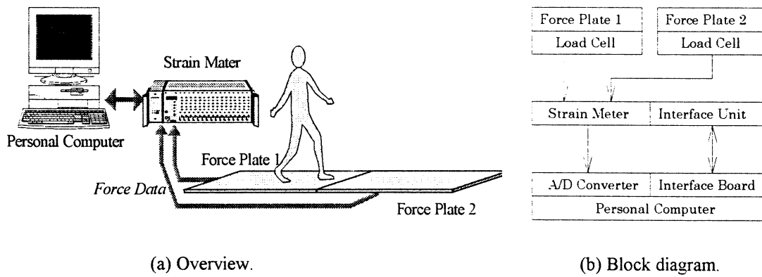
Figure 1. Experimental system for measuring.
