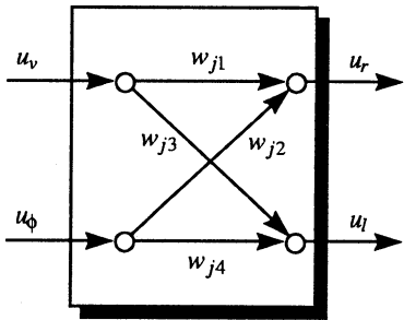
Figure 13: Jacobian net: unknown case
