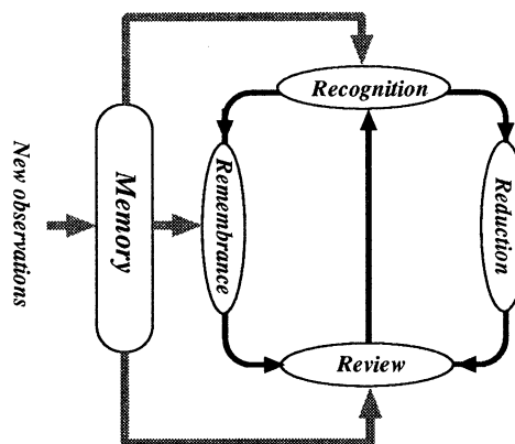
Figure 1: R^4 -rule for evolutionary learning
