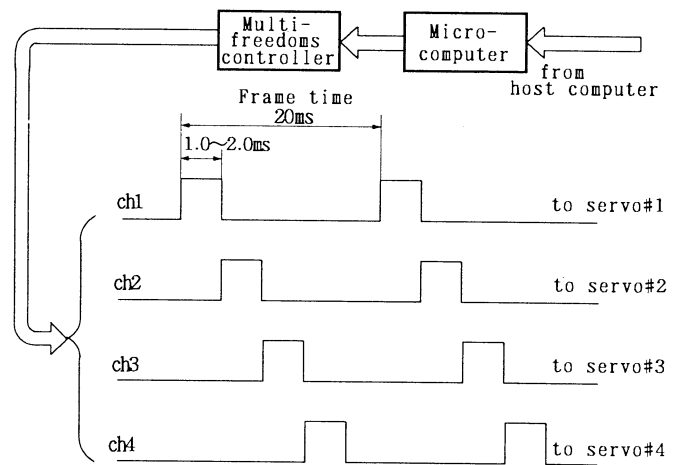
Figure 3: Input pulse to servo-mechanism
