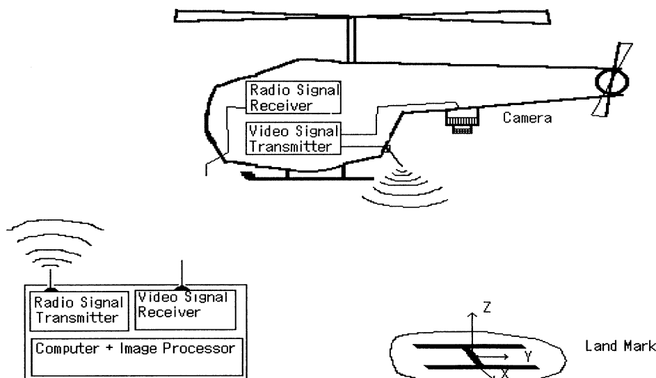
Fig.1 Configuration of Helicopter System
