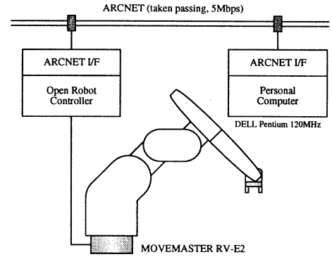
Fig. 5: An open architecture robot system.
