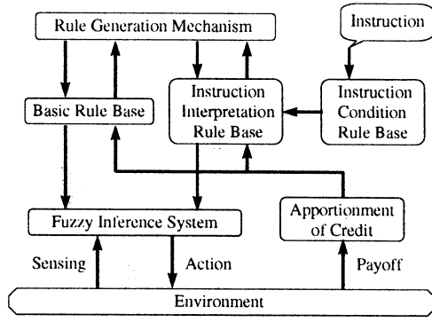
Figure 1: Fuzzy Classifier System in [6.7]
