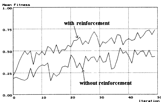
Fig. 5 Fitness changes versus iteration
