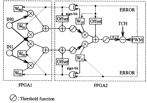
Figure 6: 2 input 1 output neural network
