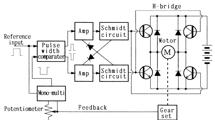
Figure 4: Servo mechanism
