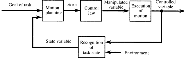
Fig. 1: Block diagram of the feedback control applied to a robotic task.
