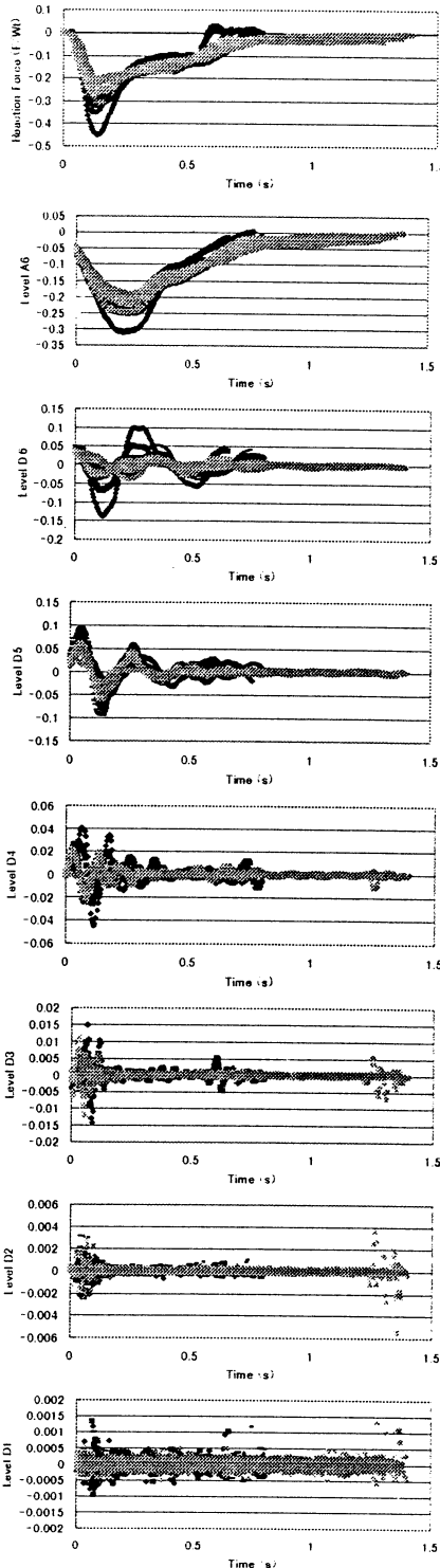
Figure 5. Comparison between F_x in stopping and F_x in changing direction. (▨ : Stopping, ■ : Changing direction)
