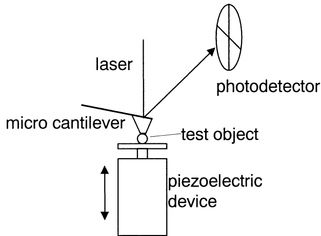
Fig.1 Schematic diagram of dynamic viscoelasticity measuring system
