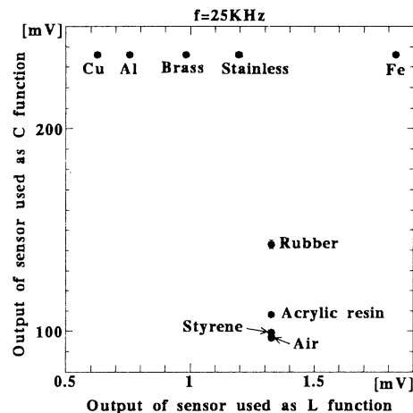
Fig. 6: Experimental results in capacitive and inductive function of comb shaped touch sensor
