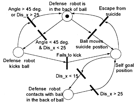
Figure 11: Petri-net model for defense controller.
