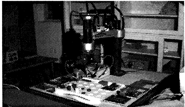
Fig. 6 The Experimental equipment set-up.
