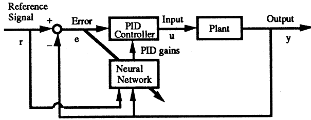
Fig. 2. Self-tuning neuro-PID control scheme.
