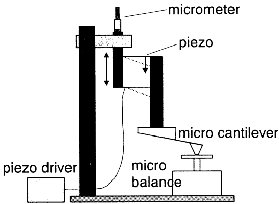
Fig. 5 Precision micro balance and piezoelectric device were applied for measuring spring constant of micro cantilever
