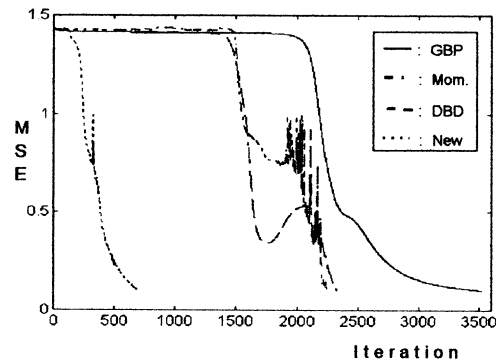
Fig. 1 Comparison of convergence using the learning parameters of first case in Table 1.
